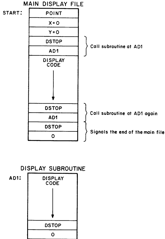
Figure 9 Subroutining Example
